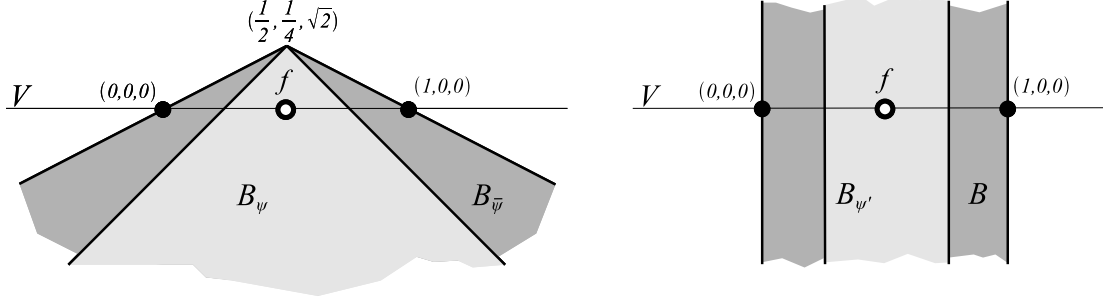
Figure 2: Lattice-free sets in the 2-dimensional space W .
