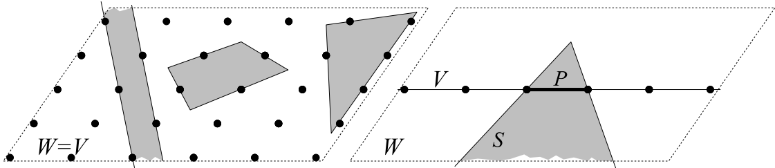
Figure 1: Maximal lattice-free convex sets in a 2-dimensional subspace (Theorem 1(i)).
