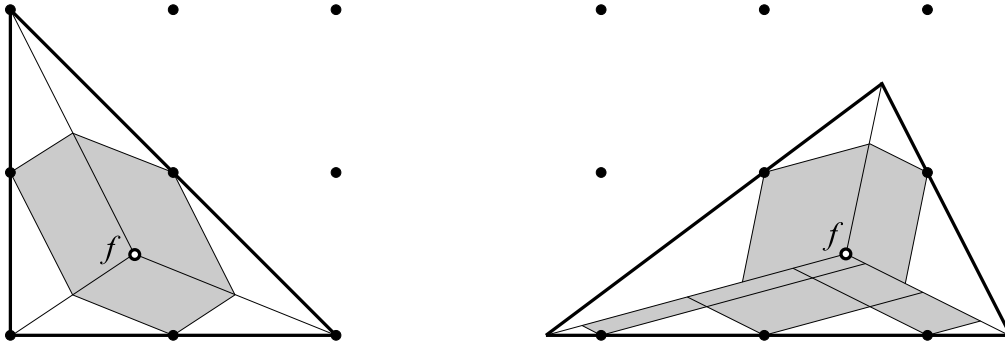
Figure 4: Lattice free triangles giving inequalities with a unique minimal lifting. Region R + \{f\} is shaded.
