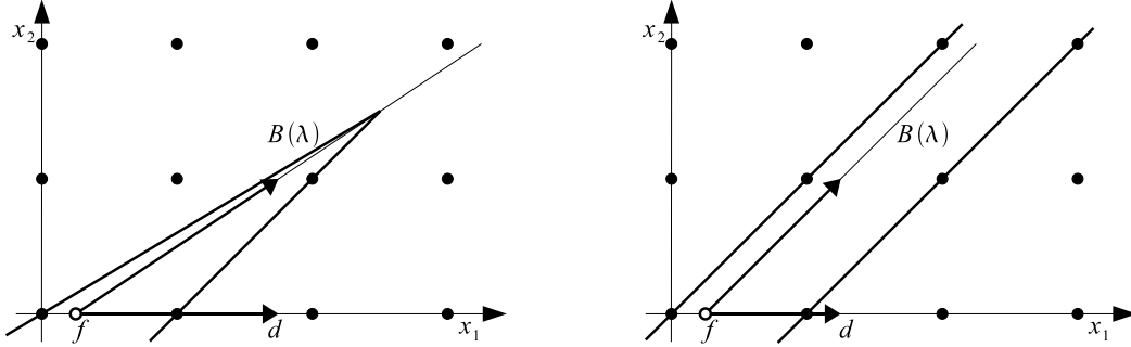
Figure 1: Example: f = \frac{1}{4} . Left: d = \frac{3}{2} . Right: d = 1 .
